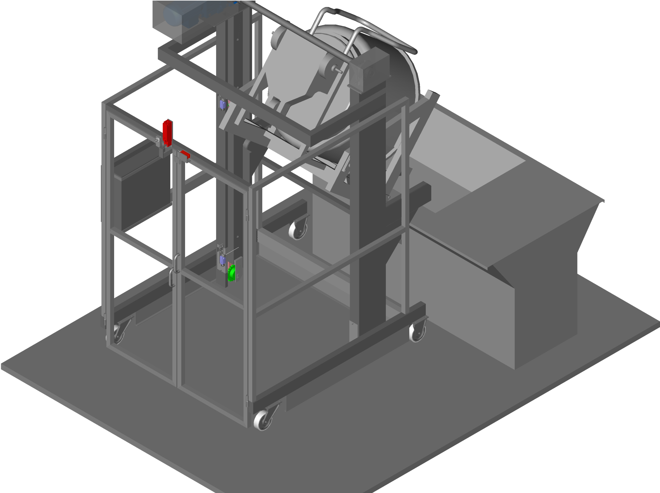
Filename: 3D MODEL OF BOWL TIPPER IN FULL TIP POSITION.pdf
